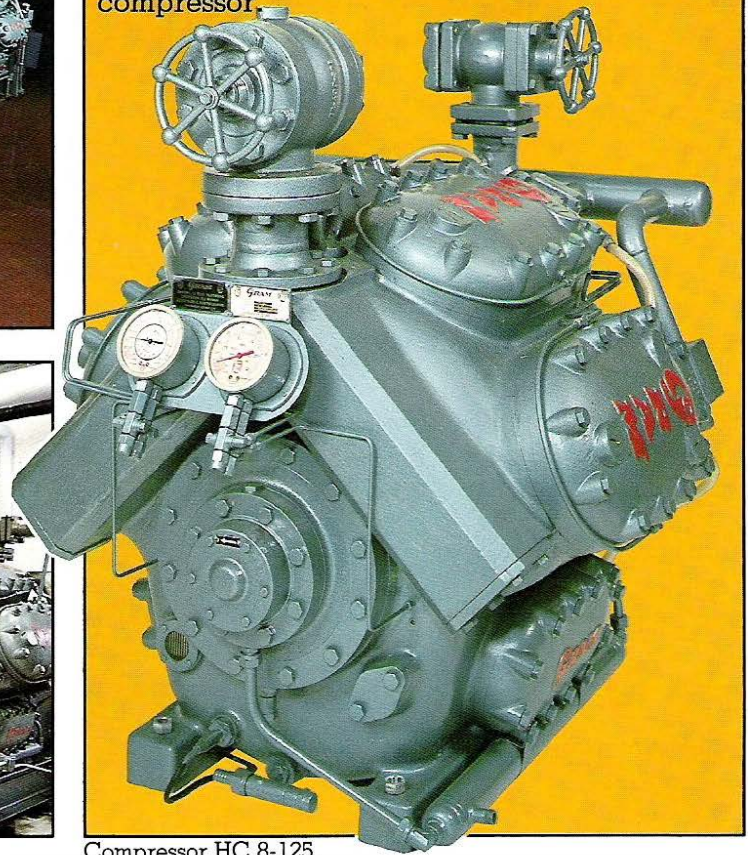
Compressor HC 8-125.
