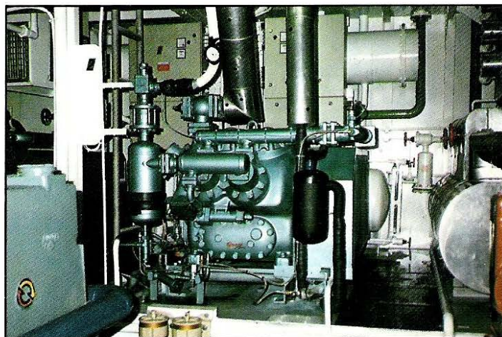
Marine refrigerating plant for shrimp freezing in Australia.
